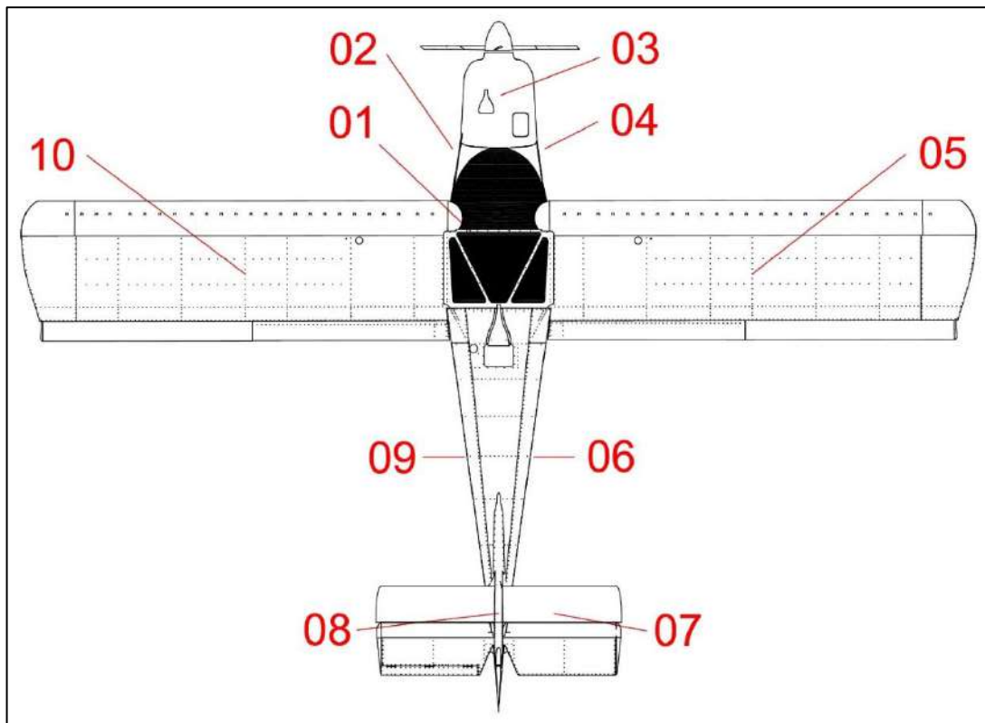
Figure 9: Daily pre-flight check sequence plan view
