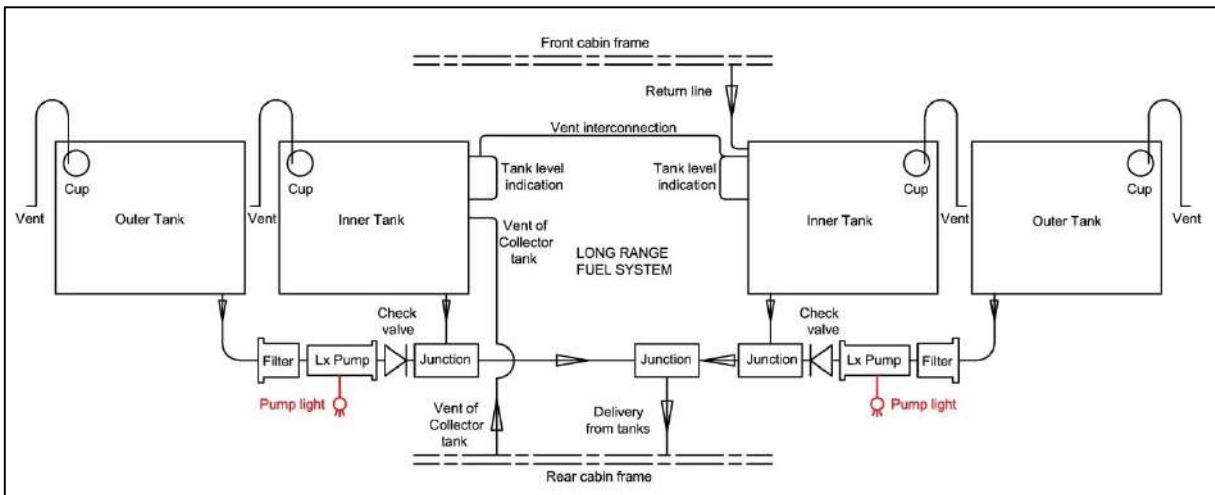
Figure 25: Wing double fuel tank system with transfer pumps
