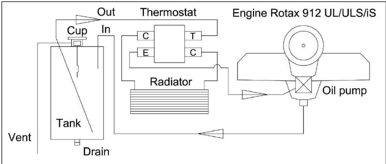
Figure 29: Rotax 912 UL/ULS/iS oil system with thermostat
