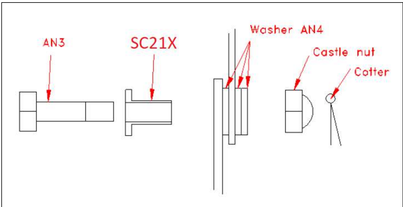
Figure 46: Control surfaces hinges
