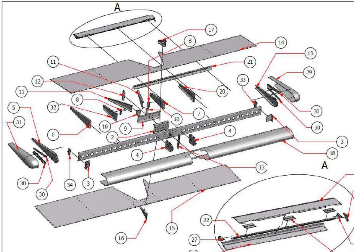
Figure 18: Elevator
