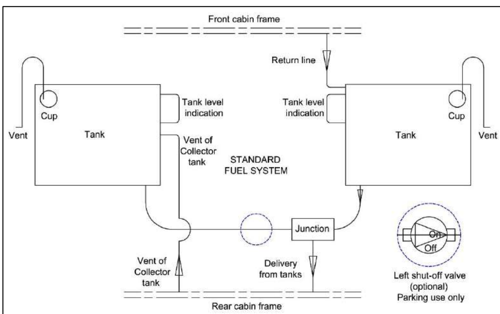
Figure 23: Wing standard fuel system
