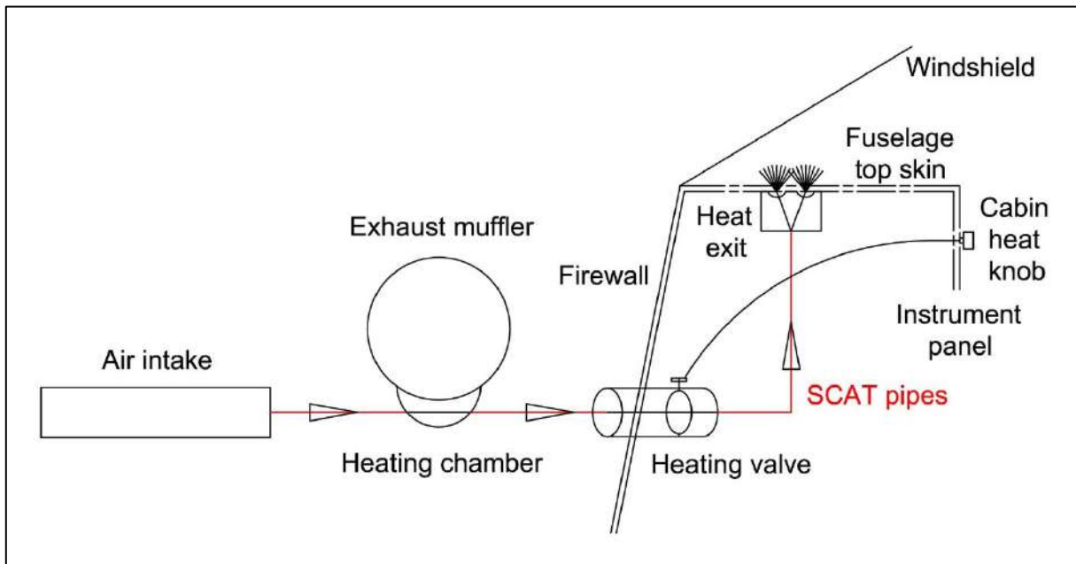
Figure 35: Cabin heating system
