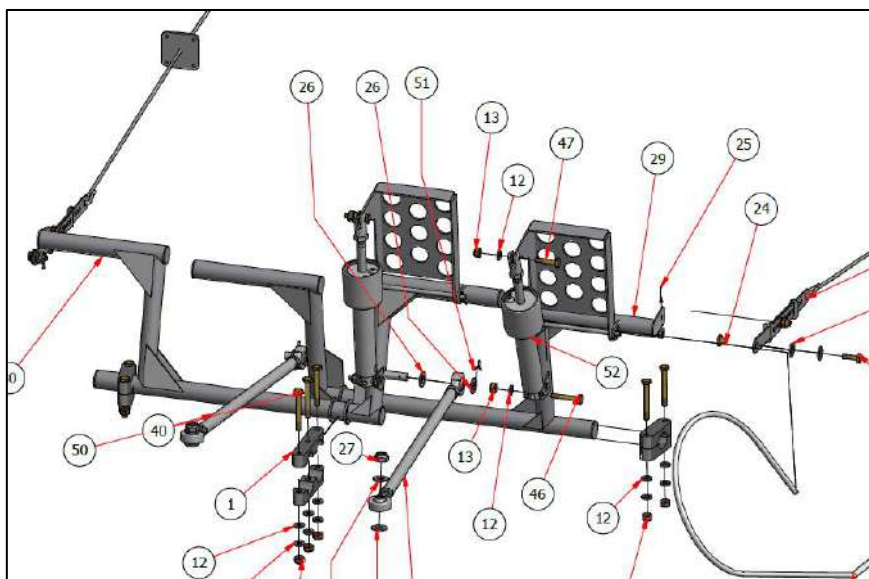
Figure 21: Directional controls
