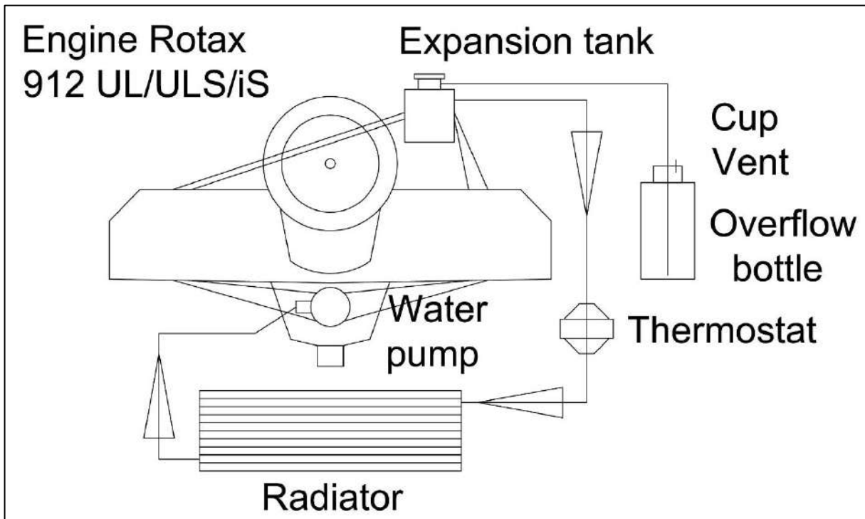
Figure 31: Rotax 912 UL/ULS/iS cooling system with thermostat
