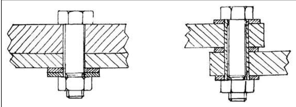
Figure 3: Threaded fasteners
