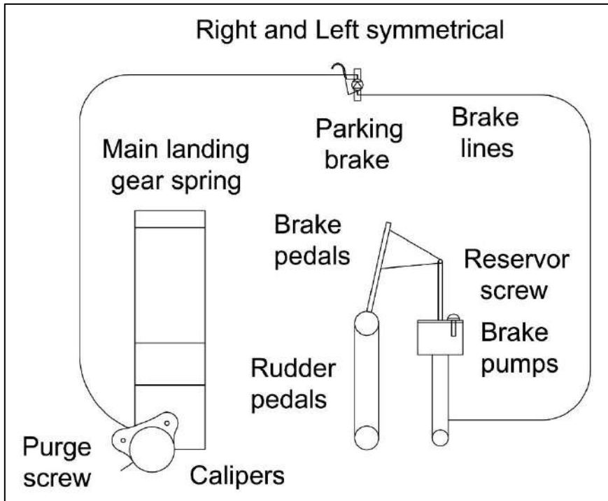
Figure 33: Brake system with parking brake (only right side is shown, the left is identical, symmetrical)
