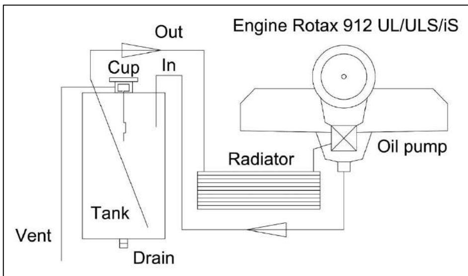
Figure 28: Rotax 912 UL/ULS/iS standard oil system
