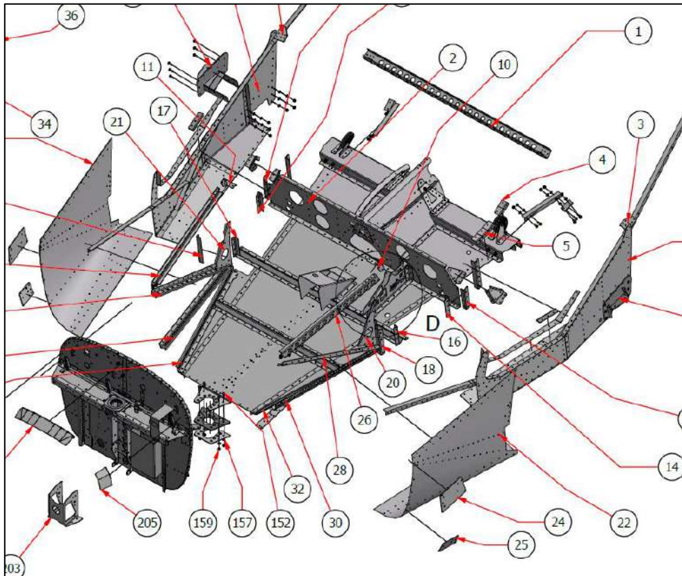
Figure 11: Cabin floor
