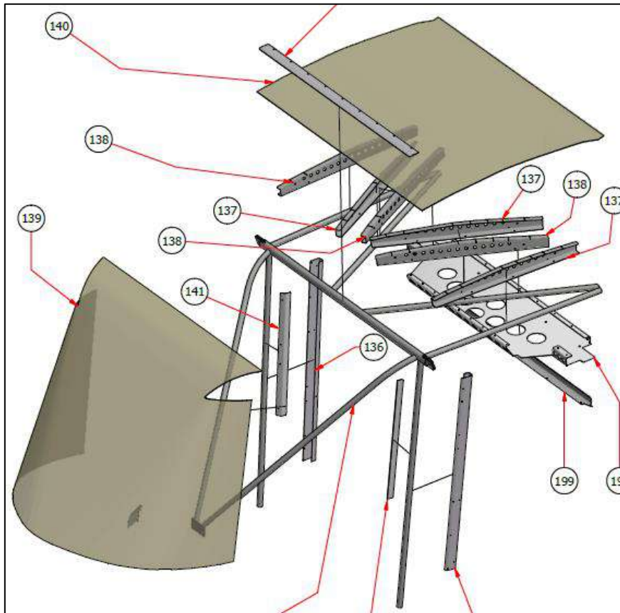
Figure 13: Cabin frame and windshield
