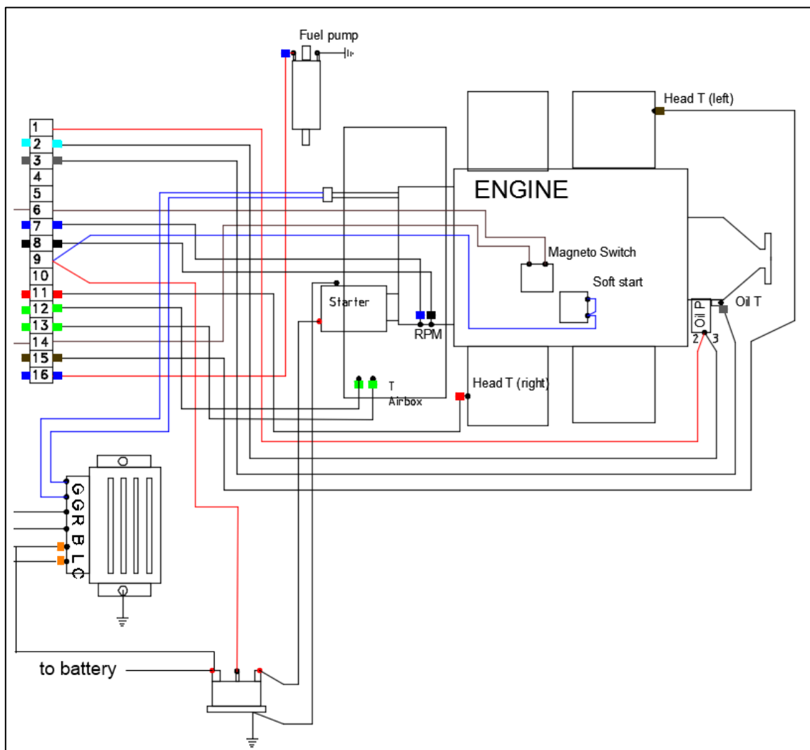
Figure 36: Electrical wiring of engine compartment
