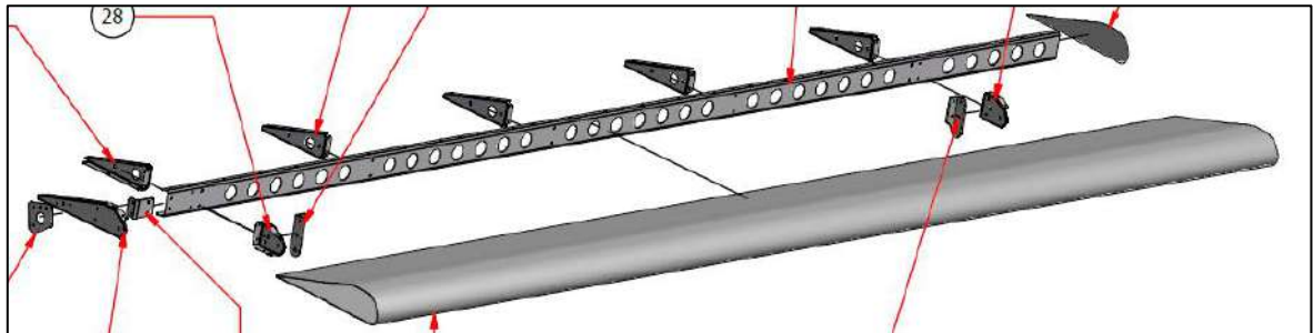
Figure 16: Left outboard flaperon
