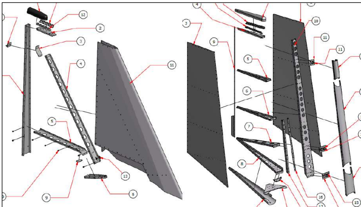
Figure 19: Fin and Rudder
