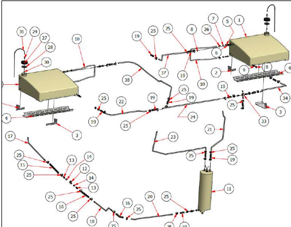
Figure 22: Airframe fuel system parts
