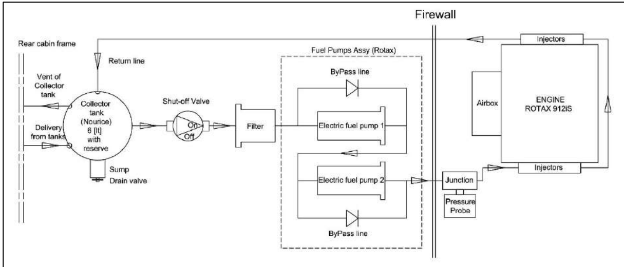
Figure 27: Fuselage Rotax 912 iS fuel system
