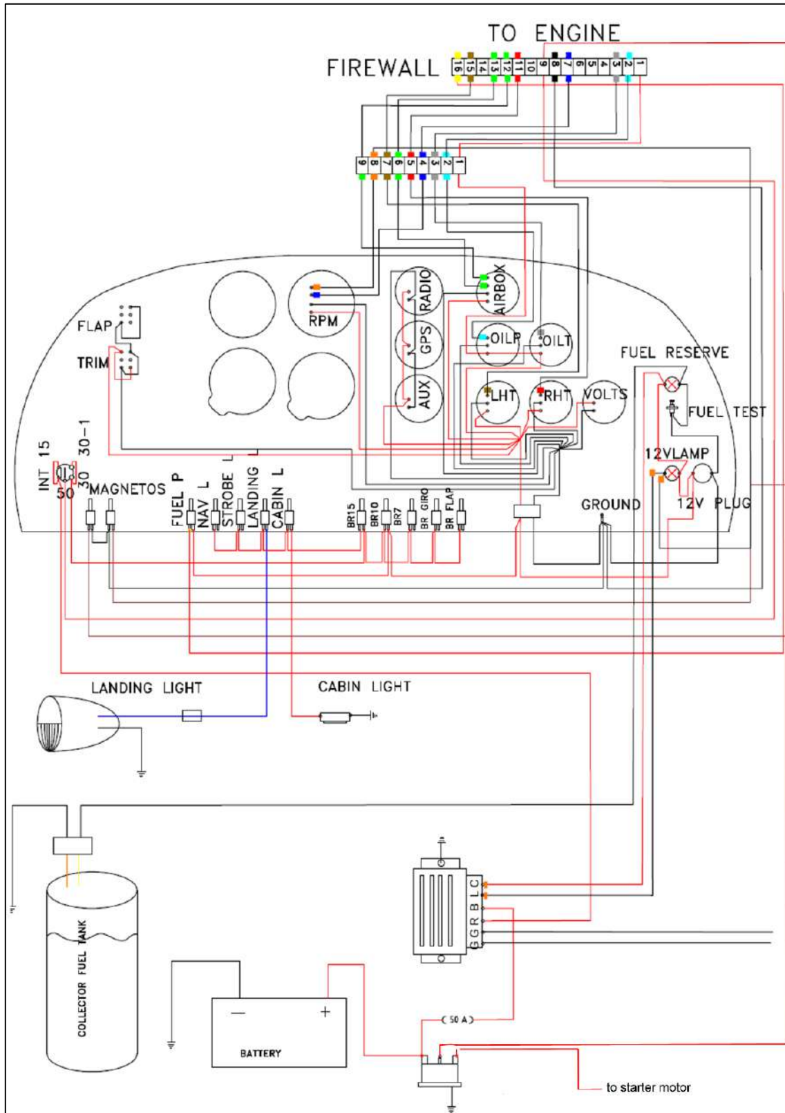
Figure 37: Electrical wiring firewall backward
