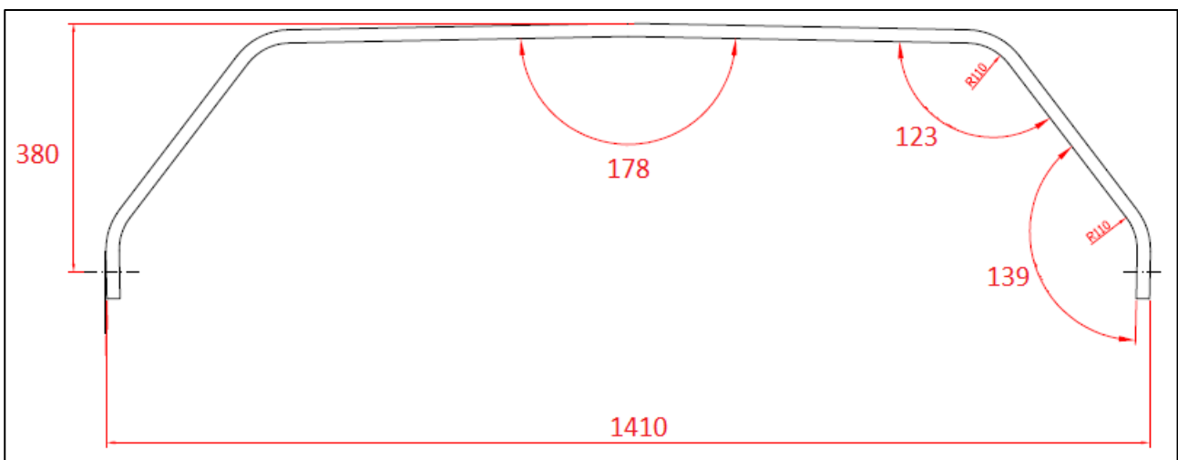
Figure 10: Main landing gear spring design nominal dimensions (unloaded)
