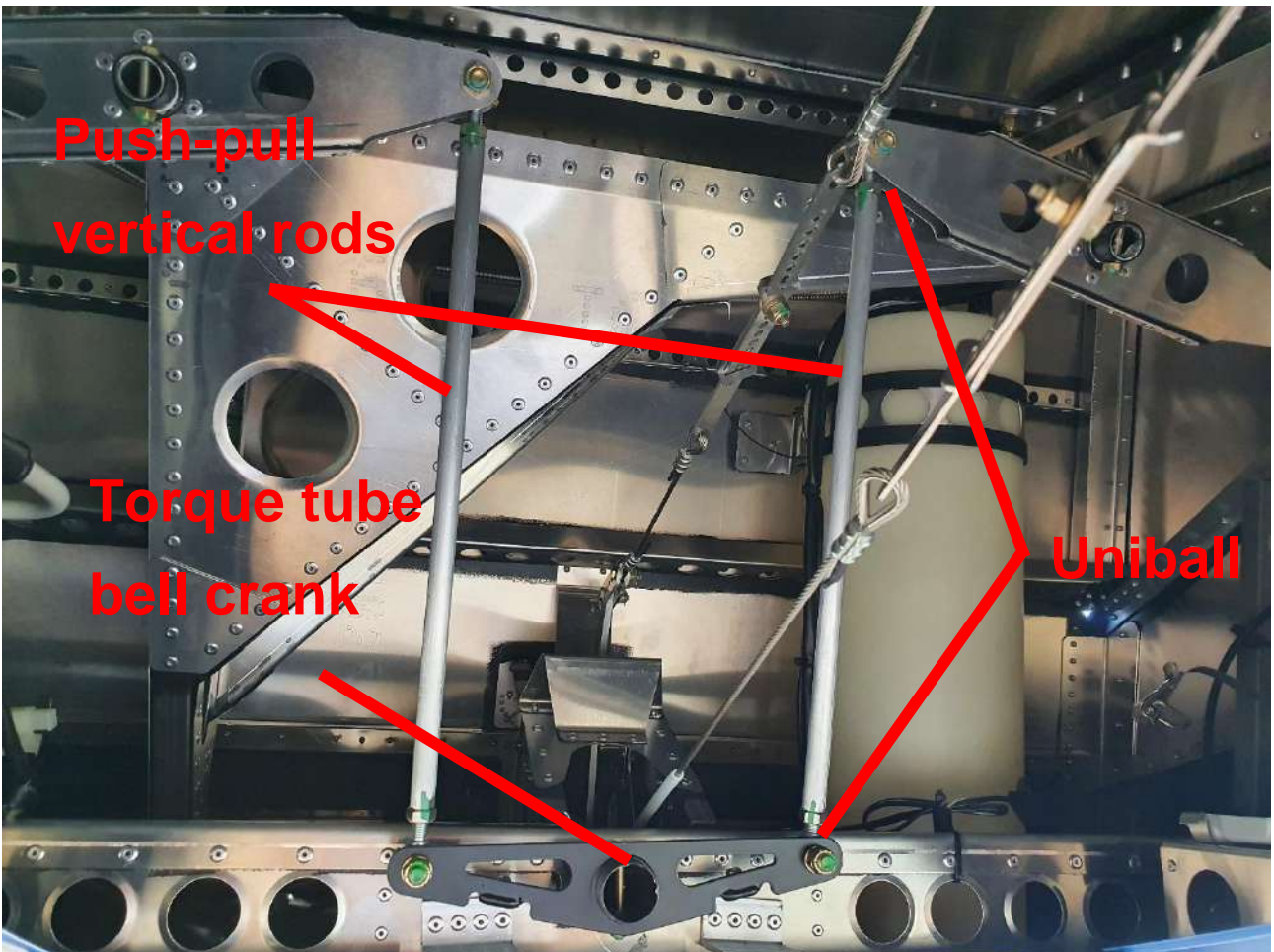
Figure 41: Push-pull rods for Flaperon setup
