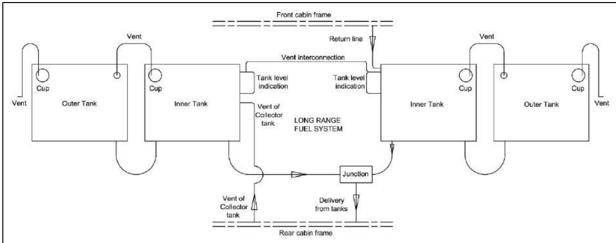
Figure 24: Wing double fuel tank system (interconnected tanks)
