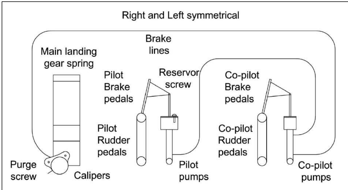
Figure 34: Double side brake system (only right side is shown, the left is identical, symmetrical)
