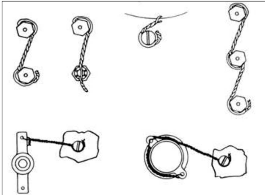
Figure 1: Safety wires example
