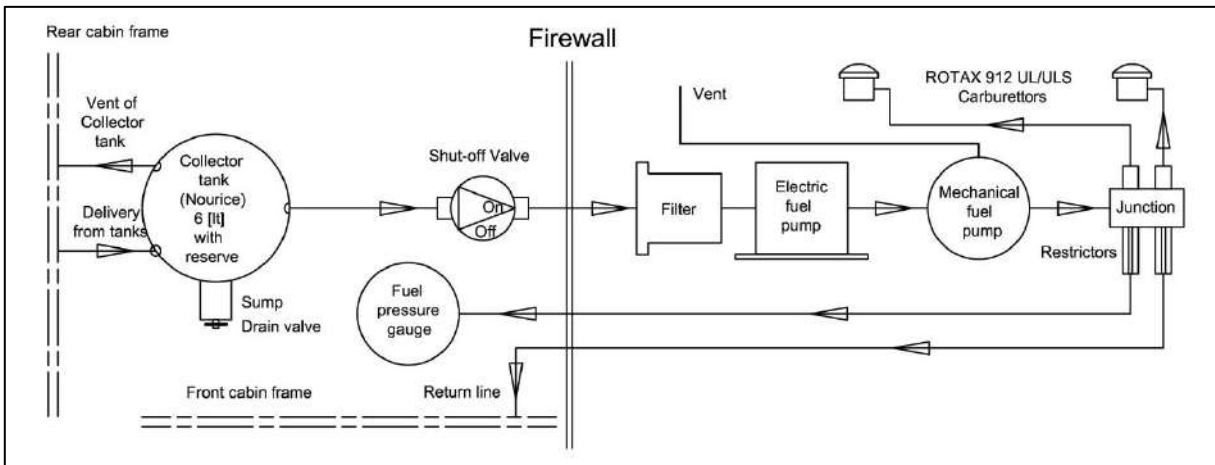
Figure 26: Fuselage and Rotax 912 UL/ULS fuel system
