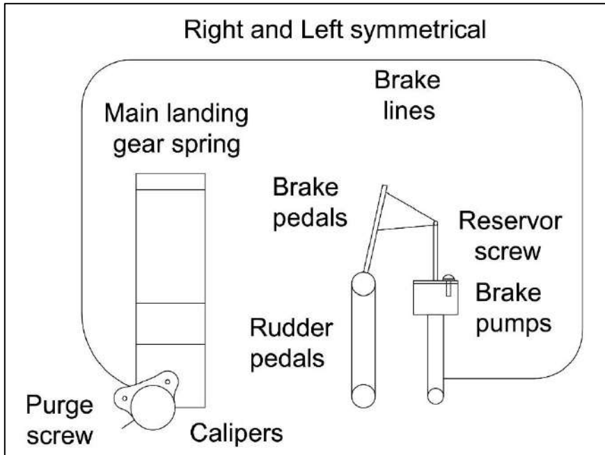
Figure 32: Standard brake system (only right side is shown, the left is identical, symmetrical)
