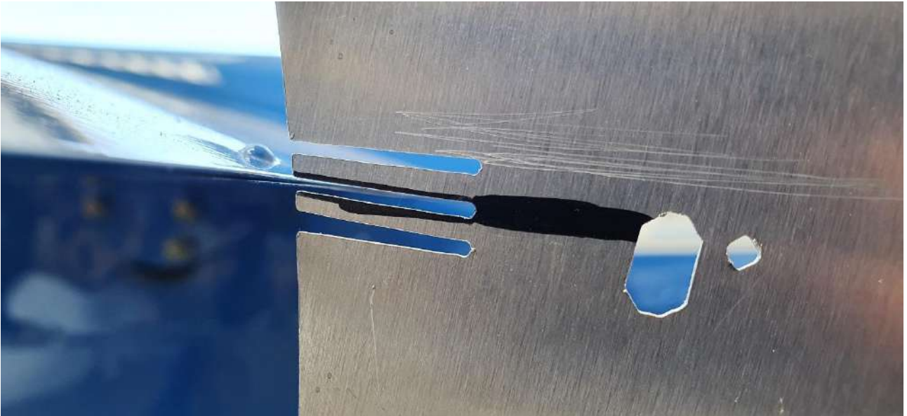
Figure 40: ZERO setting of the left inner Flaperon. Marks of +/- 0.5° of tolerance
