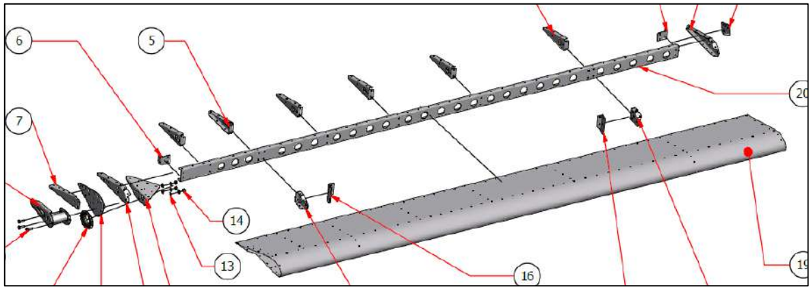
Figure 15: Left inboard flaperon
