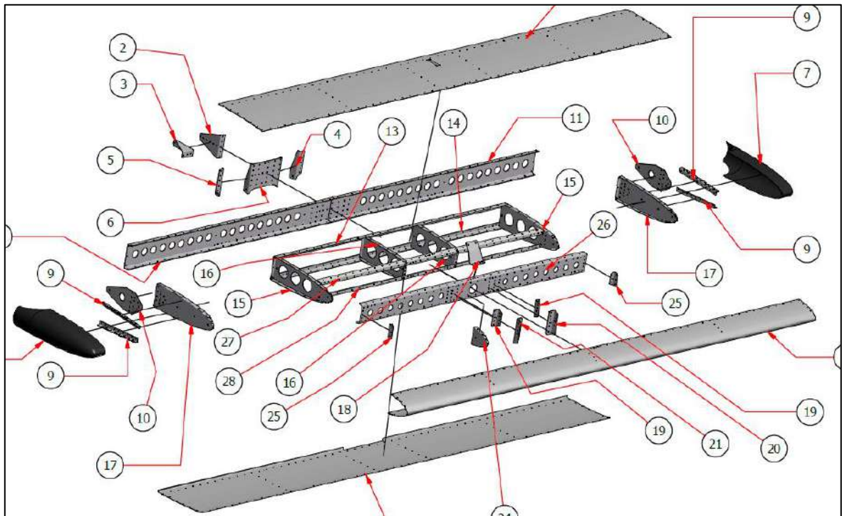
Figure 17: Stabilizer
