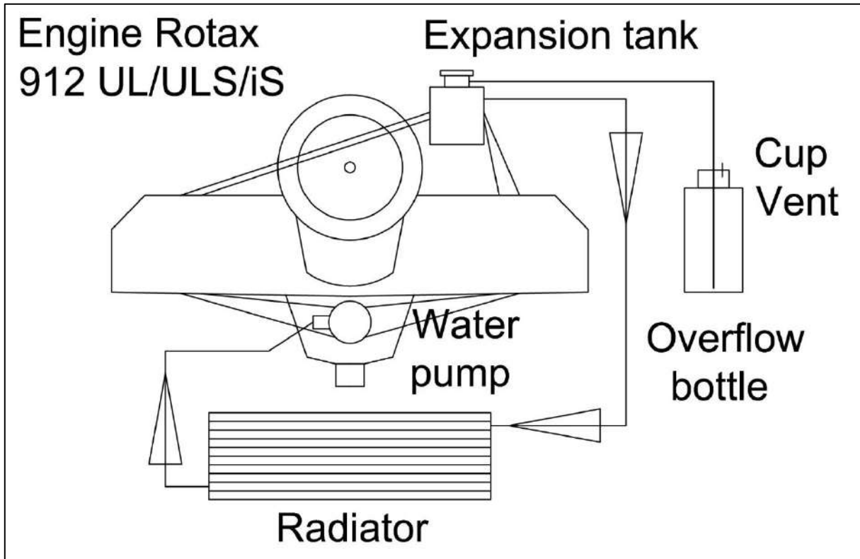
Figure 30: Rotax 912 UL/ULS/iS standard cooling system
