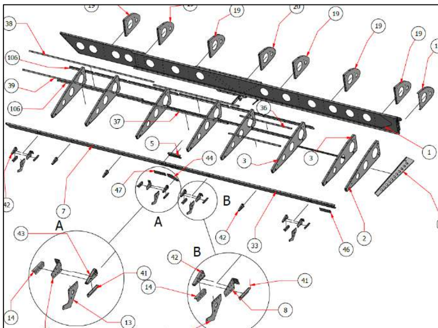
Figure 14: Left wing
